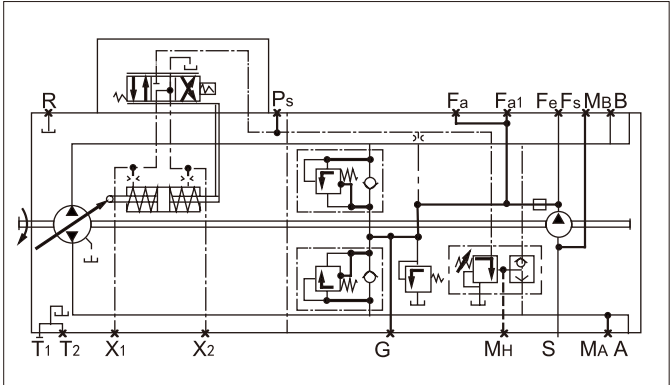
Hydraulic schematic diagram
